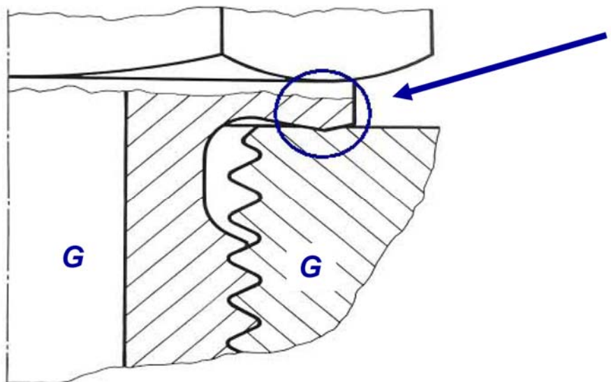
Fig. 1: Detailed drawing of sealing edge principle
